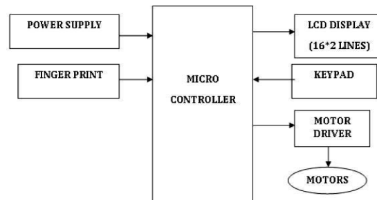
Figure 1: Block Diagram
