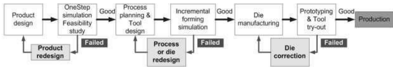
Fig.3 Workflow in simulation based process planning and die design
