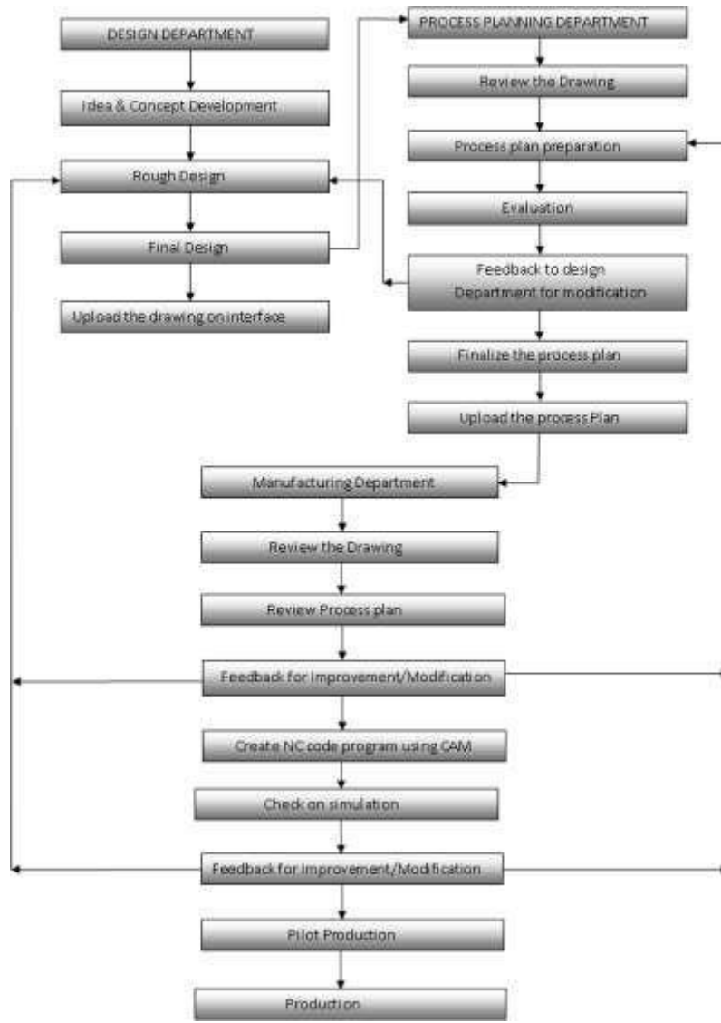
Fig4: Work flow in proposed system
